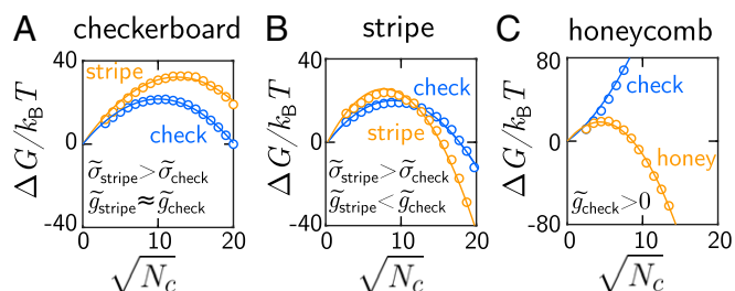
Fig. 5. Gibbs free energy G versus crystal size N_c for the free-energy landscapes in Fig. 4. Blue circles and lines correspond to checkerboard crystals; orange circles and lines correspond to stripe ( A and B ) or honeycomb ( C ) crystals. Free energies are calculated by integrating the Boltzmann weights in Fig. 4 D-F over \Phi at fixed N_c . Lines are quadratic fits of Eq. 2. \tilde{\sigma} is the effective surface free-energy density and \tilde{g} is the effective bulk free-energy density. Subscripts indicate the corresponding lattice structure. The binding free energies are E_{AA} = E_{BB} = 0 , E_{AB} = 7.0 k_B T ( A ), E_{AA} = 0 , E_{BB} = 1.6 k_B T , E_{AB} = 7.0 k_B T ( B ), and E_{AA} = 0 , E_{BB} = 3.5 k_B T , E_{AB} = 6.3 k_B T ( C ).
